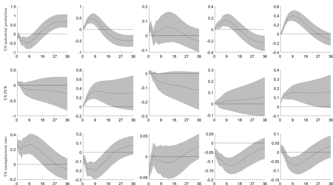
Figure A.13: PSVAR impulse response functions for US macro variables
