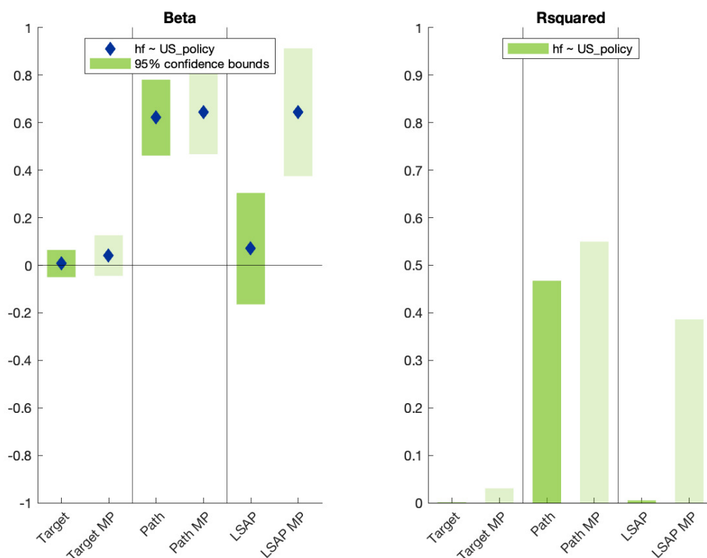
Figure B.18: US: alternative specification
