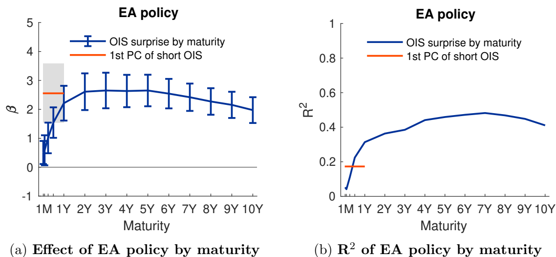
Figure 1: Explanatory power of euro area shocks for high-frequency changes in OIS rates around ECB policy announcements
