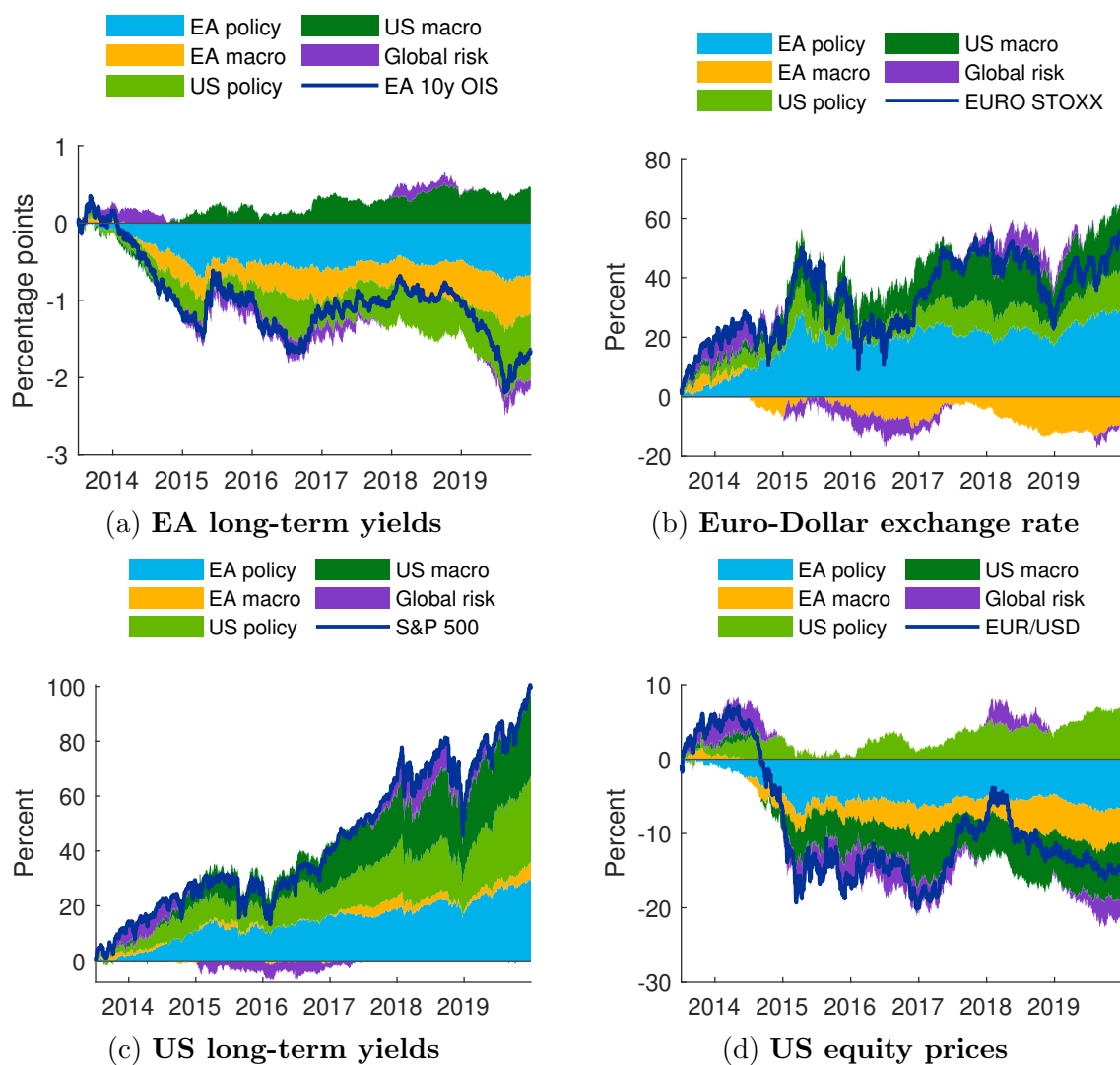
Figure A.12: Cross-Atlantic spillovers in financial markets: ECB unconventional policy 2013-2019
